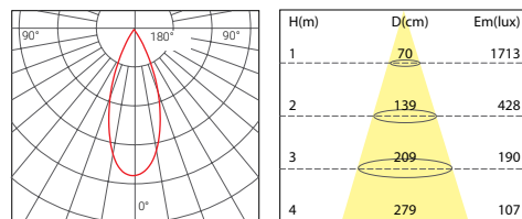
11W 40° 3000K
